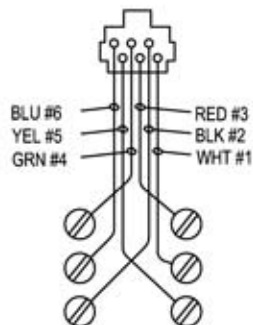
WIRING CONNECTIONS REAR VIEW
